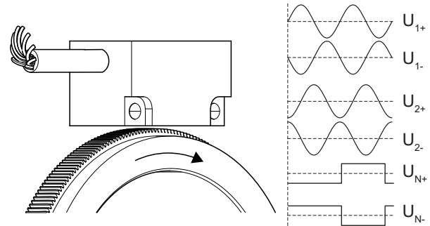
Output signals for clockwise rotation
