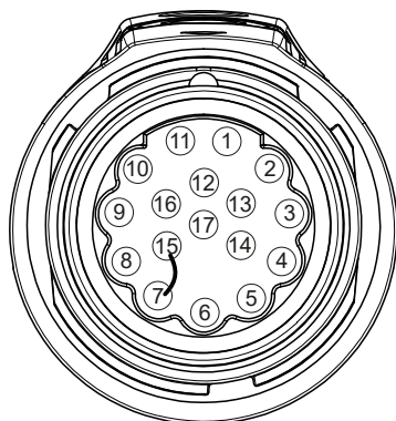
male contact (plug-in view)
